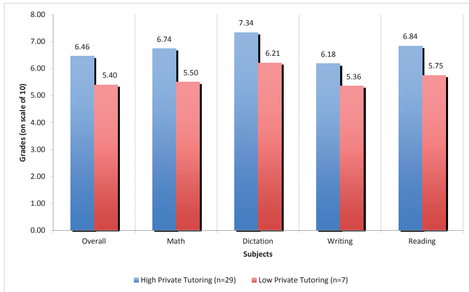
Figure 1: Score differences between high and low student attendance at private tutoring (N = 36)
